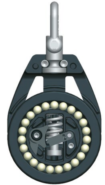
Automatic ratchet block, high load. When the load on the block increases the ratchet engages and the sheave is locked in one direction.
